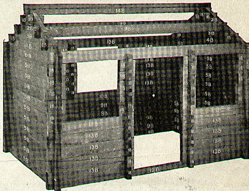
LINCOLN PLAYHOUSE ROOF REMOVED TO SHOW CONSTRUCTION
