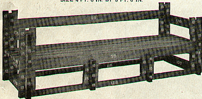
BENCH BUILT FROM PLAYHOUSE MATERIAL
