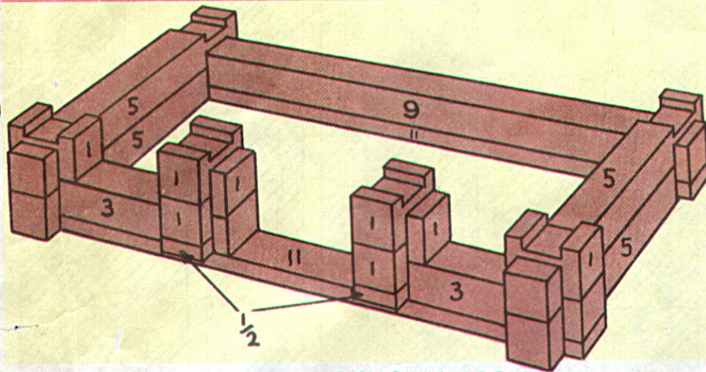
FOUNDATION PLAN IS SHOWN ABOVE
