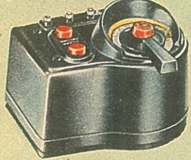
NEW — Type LW 125-Watt Transformer Offers a full range of speed for any locomotive. It also has two fixed voltages (14V and 18V) having a common ground with the track. This is very useful in case there are two different accessories connected to the track which require different voltages. Dial is illuminated. (HAS BUILT-IN CIRCUIT BREAKER)
