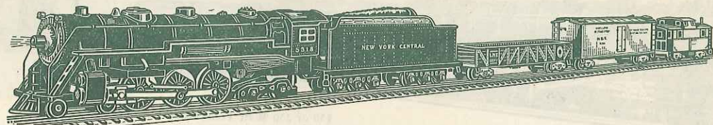
No. HO-103 — 50 or 75 Watt Transformer Recommended No. HO-103 — 3 Car Freight Train — Steam Type — Remote Directional Control Automatic Coupling — 31-In. Long
